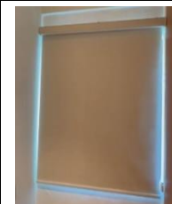
FOC High Temperature Shaping
